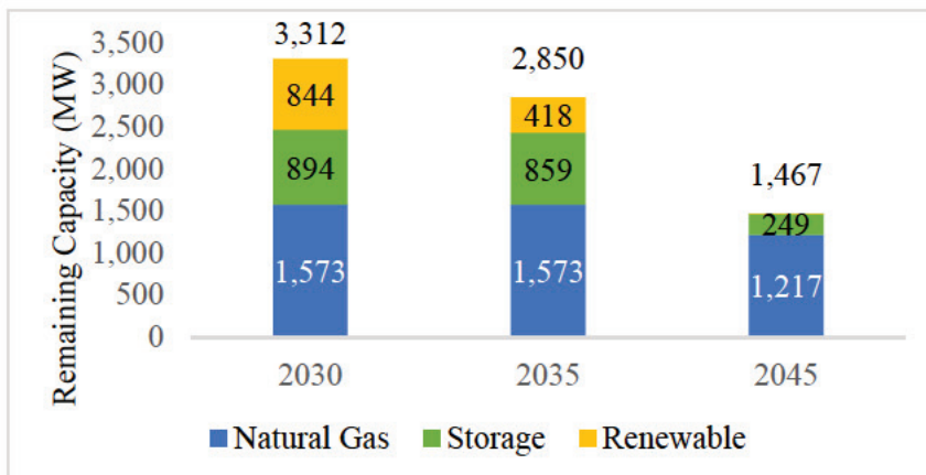
Figure 1 SDG&E Current Owned or Contracted Portfolio Resources by Year (Nameplate MW)
