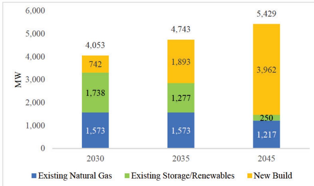
Figure 2 Existing and Incremental Procurement Requirements by Year (Nameplate MW)
