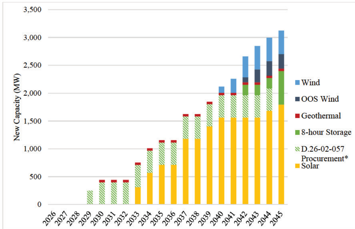
Figure 6 Alternative Portfolio Cumulative Capacity Additions by 2045
