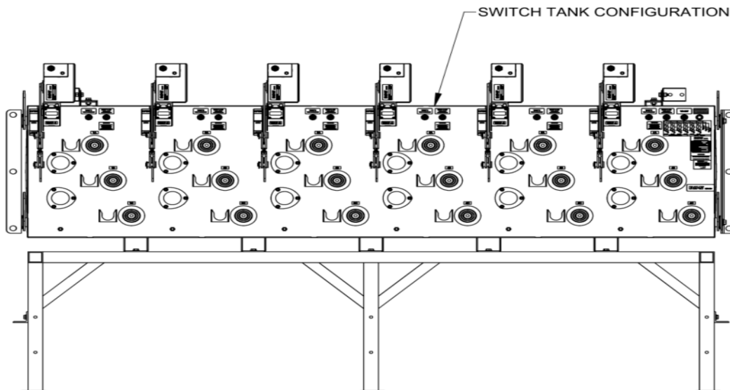
Figure 2 Walk-In Vaults Typical 6-Way Vault-Mount ISG SCADA Switch
