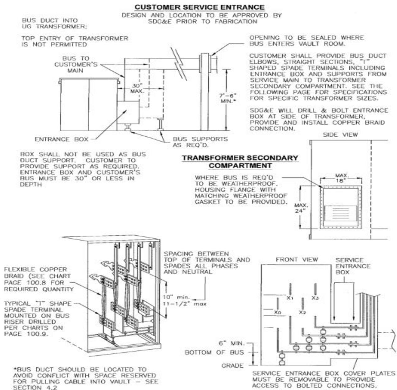
Figure 2: Typical Bus Duct Configuration for Padmounted Transformer
