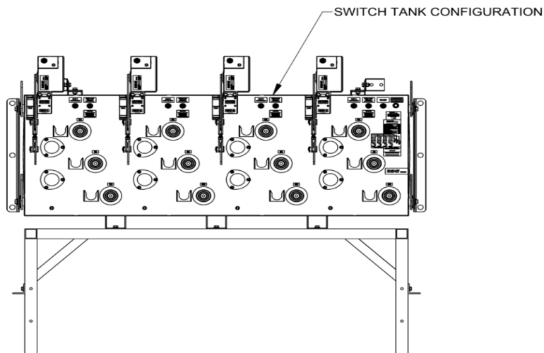
Figure 1 Walk-In Vaults Typical 4-Way Vault-Mount Vacuum Fault Interrupting Manual or SCADA Switch
