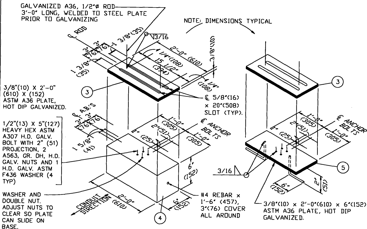
TYPE "C" SLIDING SUPPORT (NOTE: 5 1/4" LATERAL MOVEMENT) NOT TO SCALE
