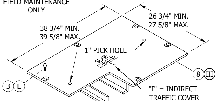
FIGURE 3 STEEL COVER FIELD MAINTENANCE ONLY (III)
