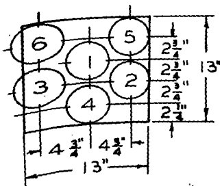
4-5" CONDUITS 4 1/2" O.D. WITH 1" SPACING AND 1" OVERHANG INTO PRIMARY SIDE SECONDARY TRANSFORMER OPENING
