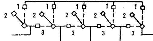
5 WAY ONE LINE DIAGRAM
