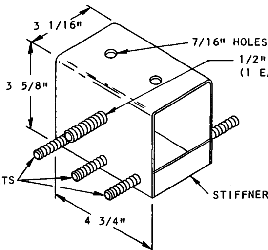
DETAIL "A" LANDING PLATE
