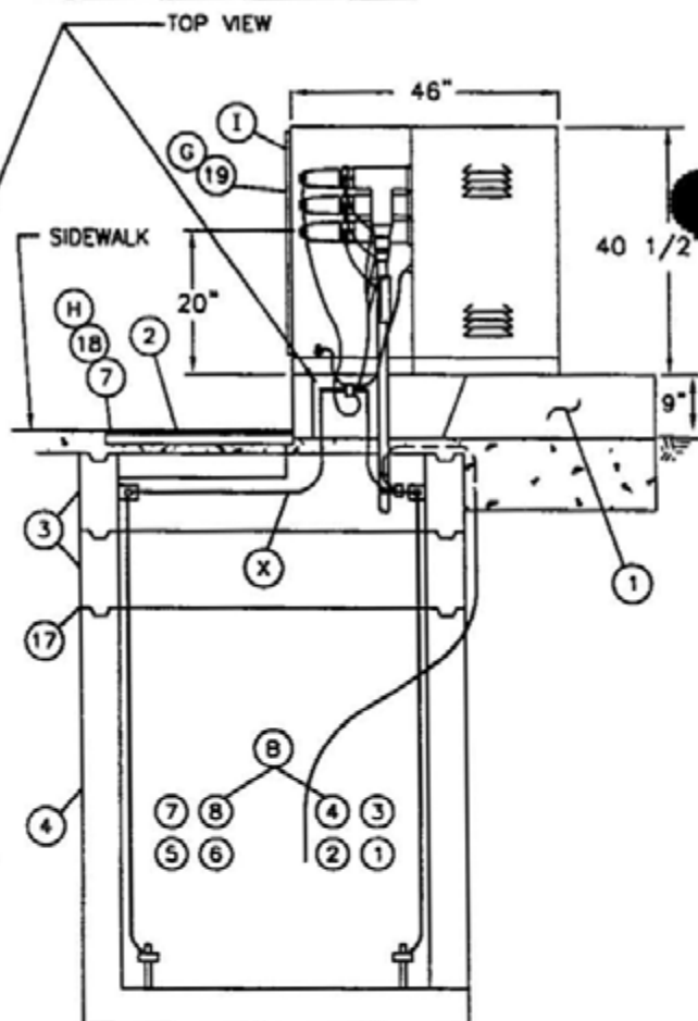
END VIEW
