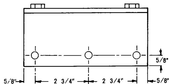
2/0 AND SMALLER SIDE
