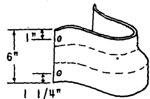
REDUCER BOOT
