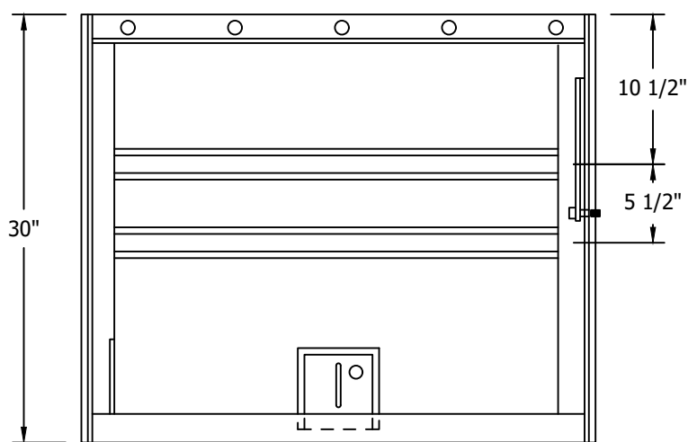
FRONT VIEW (EXPOSED)
