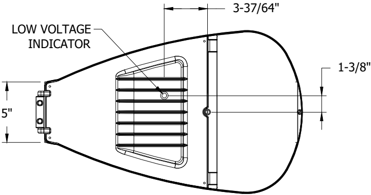
FIGURE 12 BOTTOM VIEW
