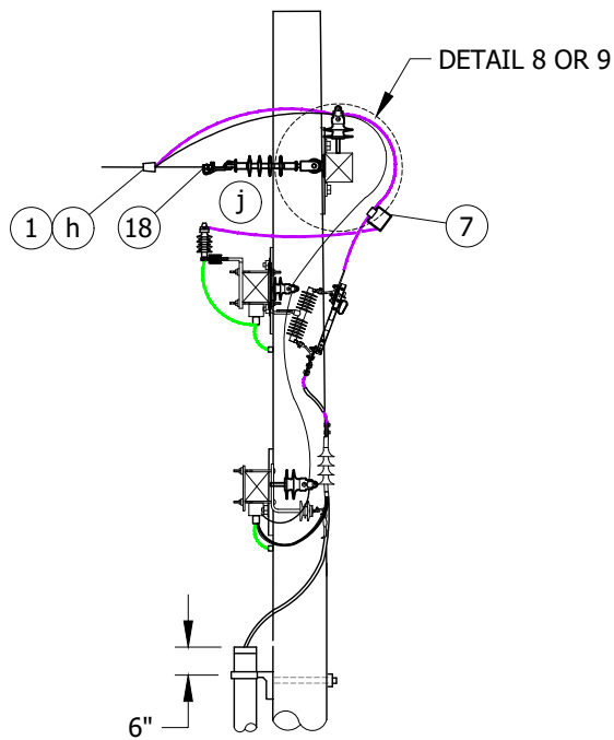
FIGURE 2 SIDE VIEW
