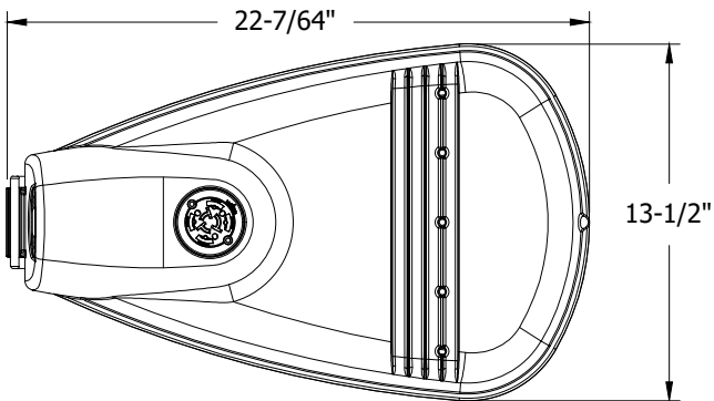
FIGURE 14 TOP VIEW
