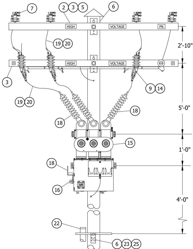
FIGURE 1 FRONT VIEW
