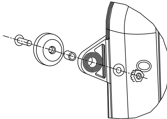
(A) FIGURE 1: MAGNETIC MOUNTING KIT ASSEMBLY
