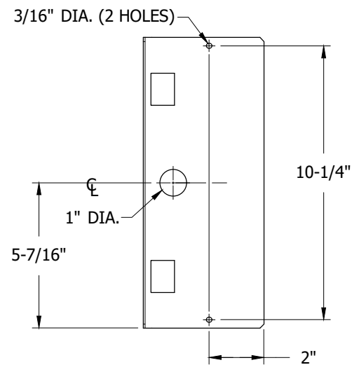
FIGURE 52 TOP VIEW
