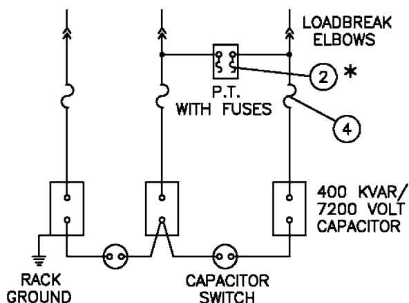
SCHEMATIC DIAGRAM
