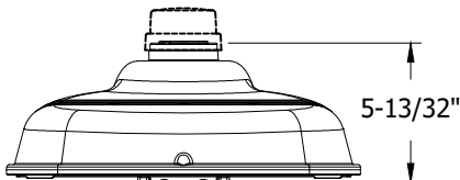
FIGURE 23 FRONT VIEW
