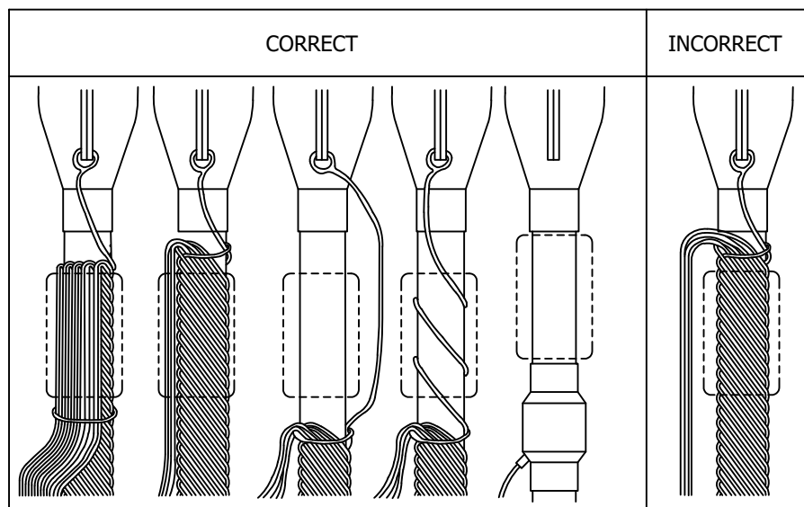
FIGURE 8: CORRECT AND INCORRECT NEUTRAL TRAINING
