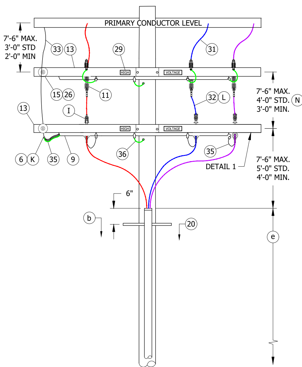
FIGURE 1 BACK VIEW OF ARM
