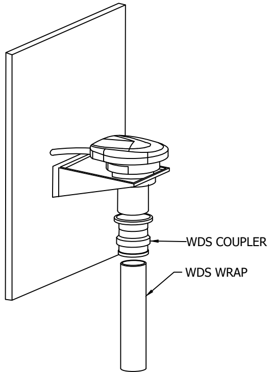
A FIGURE 20: MOUNT THE COUPLER AND TRAP TO WDS
