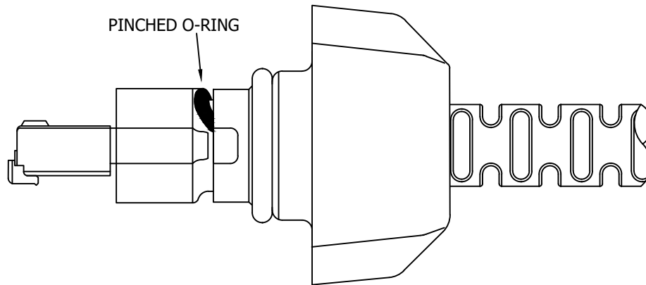
A FIGURE 22: INCORRECT INSTALL. PINCHED O-RING
