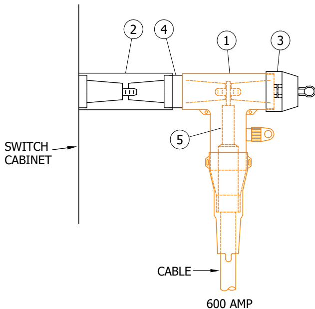
FIGURE 5 SUBSURFACE/SURFACE OPERABLE SWITCH CONNECTIONS 200 AND 600 AMP DEADBREAK
