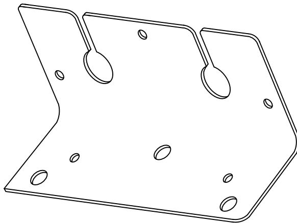
(A) FIGURE 2: REMOTE ANTENNA BRACKET
