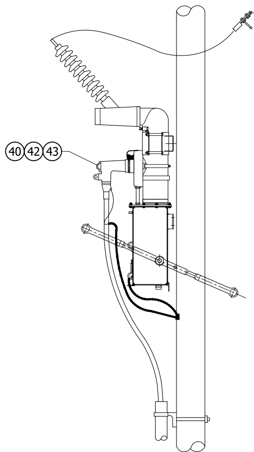
FIGURE 3 200 AMP SIDE VIEW
