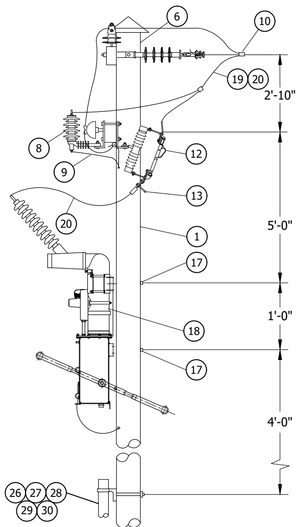
FIGURE 1 SIDE VIEW
