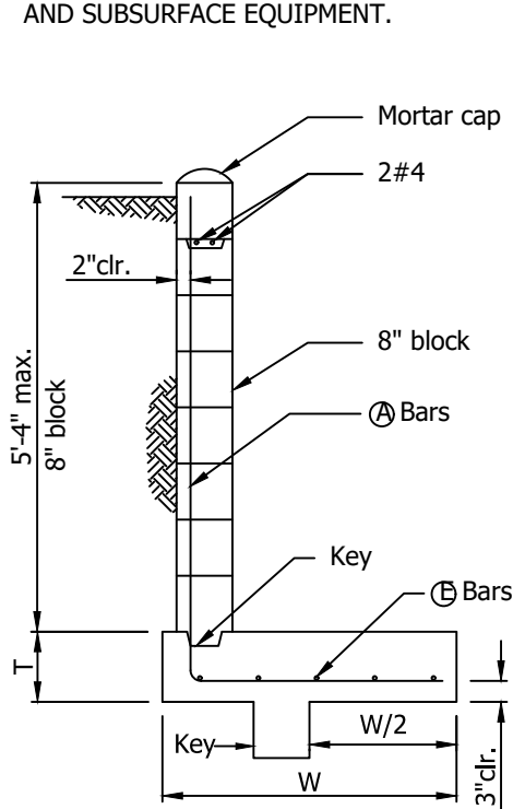
TYPICAL SECTION 5'-4" max
