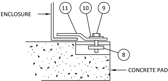
HOLD-DOWN ASSEMBLY DETAIL TYPICAL BOTH SIDES OF EQUIPMENT PAD
