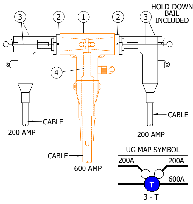
FIGURE 4 MANHOLE INSTALLATION SUBSURFACE CONNECTIONS 200 AND 600 AMP DEADBREAK
