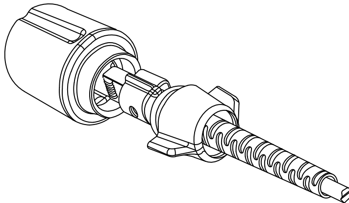
A FIGURE 20: MOUNT THE COUPLER AND TRAP TO WDS
