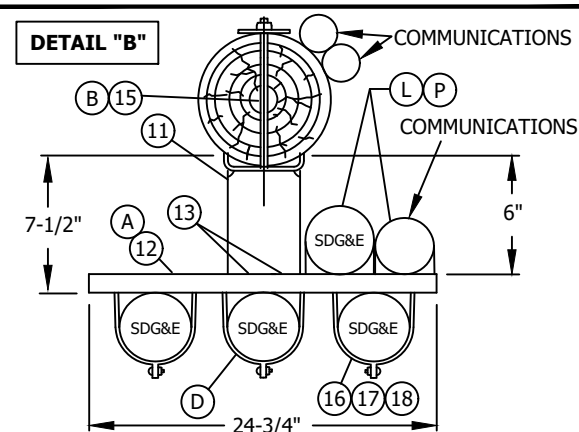
NEW MULTIPLE RISER CONSTRUCTION (SEE NOTE (H))
