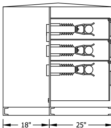
SIDE VIEW (EXPOSED)
