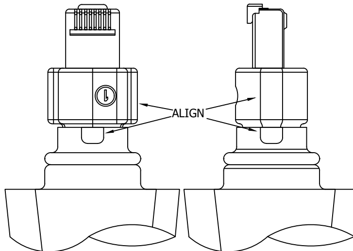
A FIGURE 23: INCORRECT INSTALL. PINCHED O-RING ENSURE THE INNER O-RING IS PROPERLY INSTALLED
