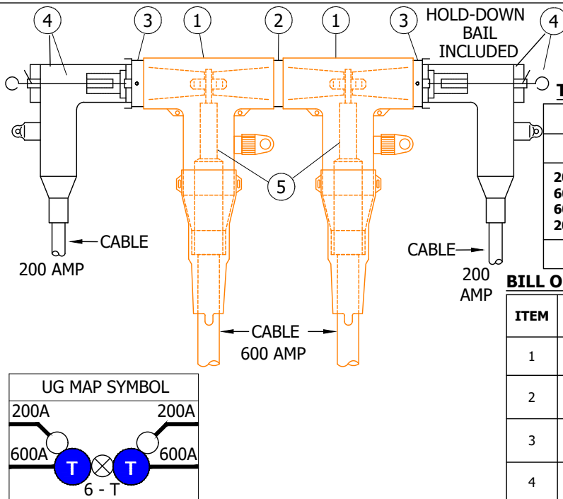
FIGURE 7 MANHOLE INSTALLATION SUBSURFACE CONNECTIONS 200 AND 600 AMP DEADBREAK
