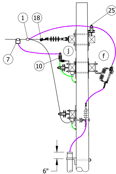
FIGURE 3 SIDE VIEW
