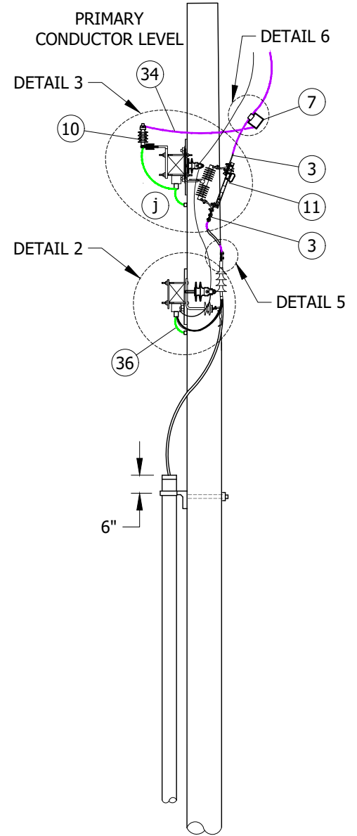
FIGURE 1 SIDE VIEW
