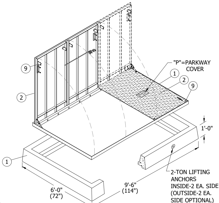
FIGURE 1 PARKWAY COVER ASSEMBLY
