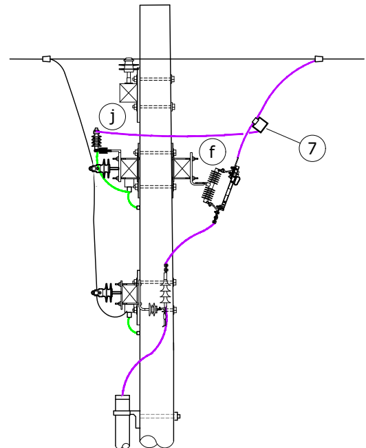
FIGURE 5 SIDE VIEW
