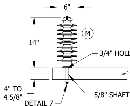
DETAIL 8 35KV F-NECK INSULATOR TANGENT OR SINGLE DEADEND ARM
