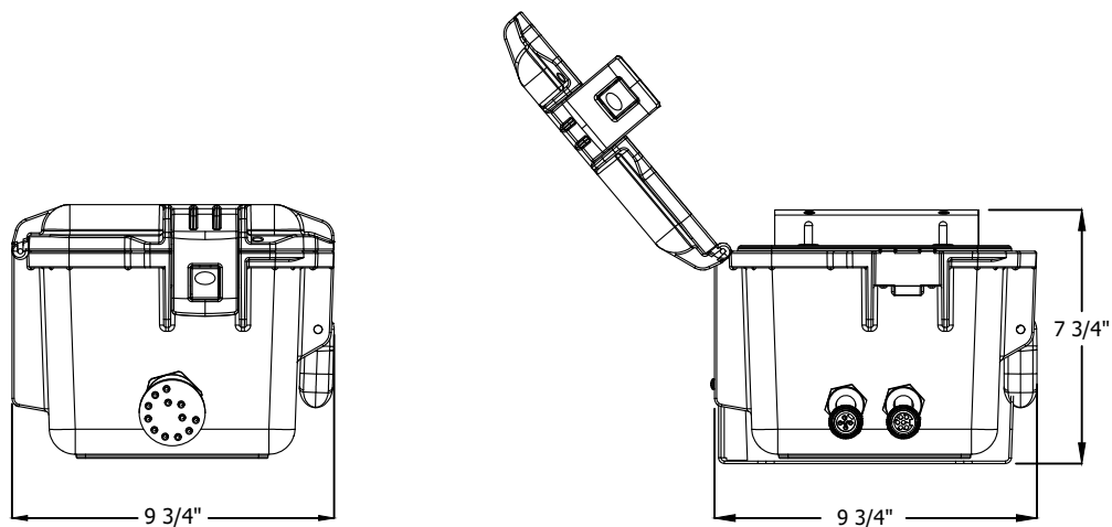
SIDE VIEWS
