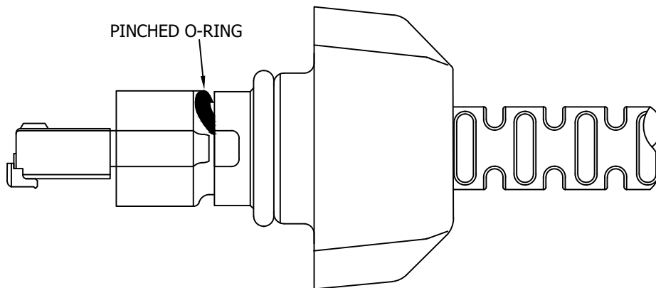
A FIGURE 13: PINCHED O-RING
