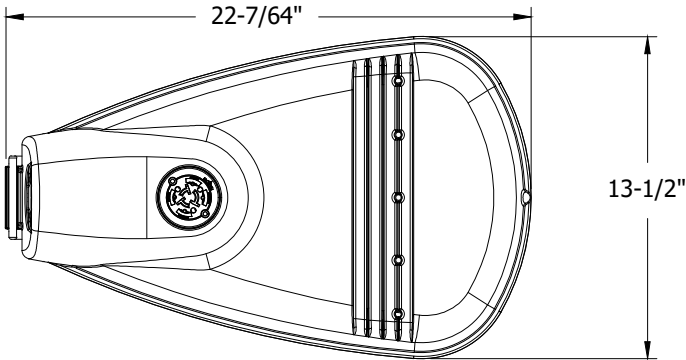
FIGURE 20 TOP VIEW
