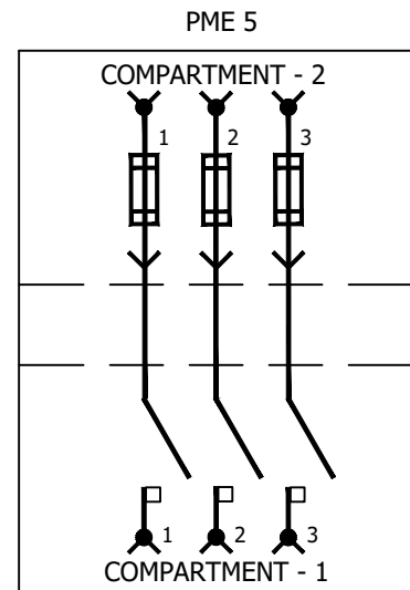
CONNECTION DIAGRAM:
