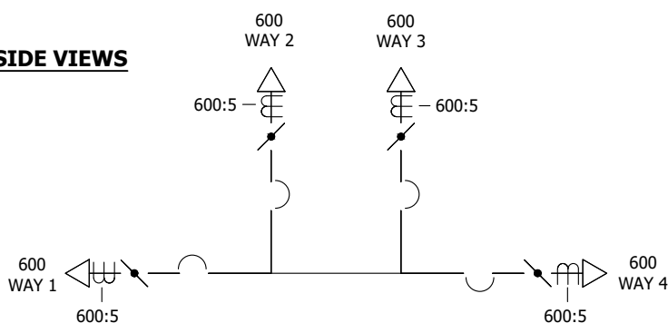
FOUR-WAY SUBMERSIBLE 600A SCADA CONNECTION DIAGRAM
