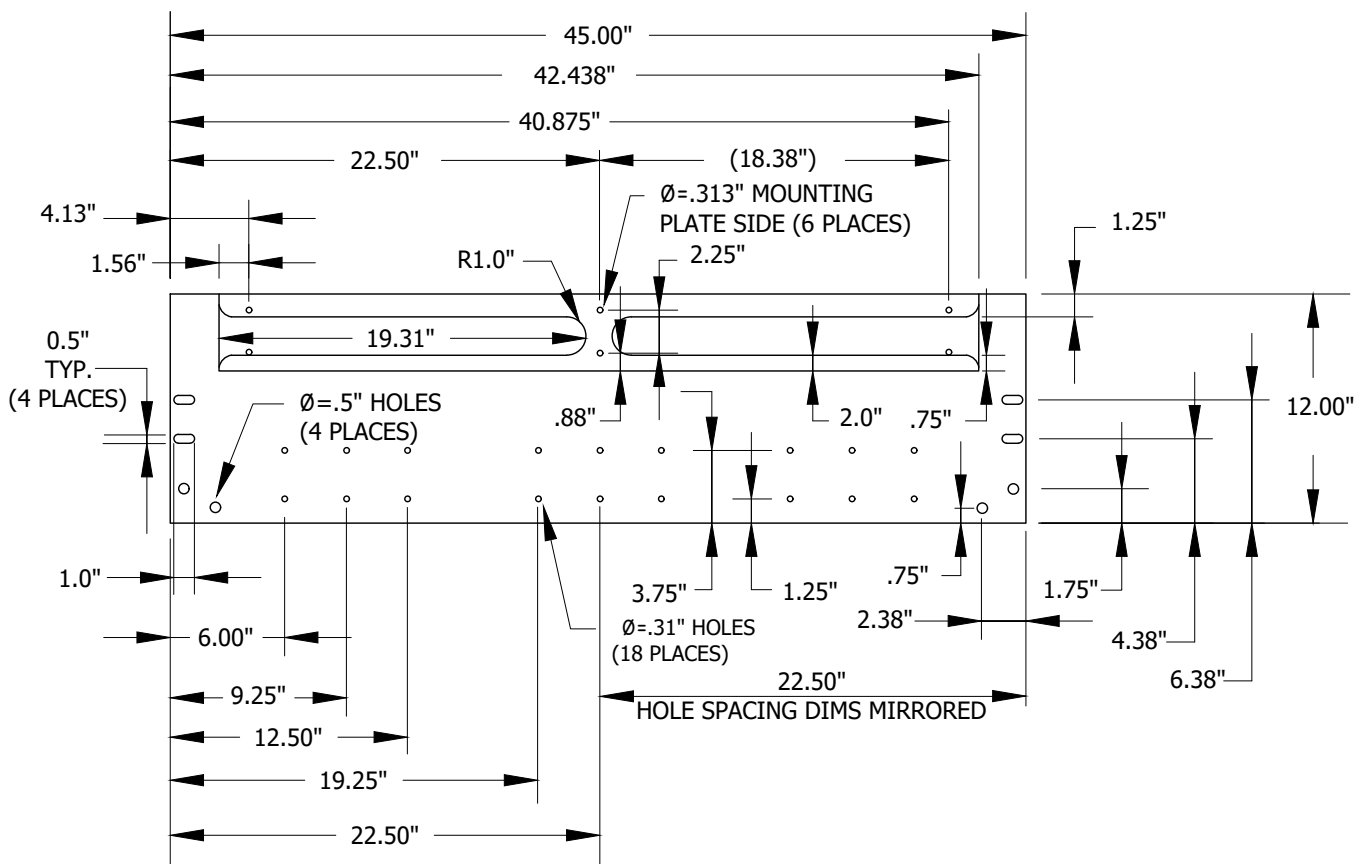
FIGURE 1 200AMP CABINET PLATE ASSEMBLY FRONT VIEW
