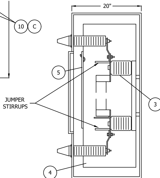
SIDE SECTION
