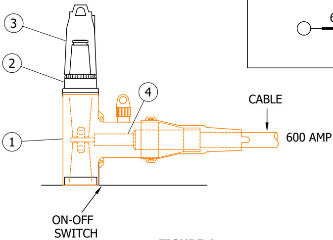
FIGURE 4 SUBSURFACE/SURFACE OPERABLE ON-OFF SWITCH 200 AMP LOADBREAK CONNECTIONS
