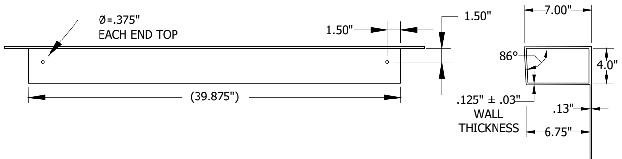
FIGURE 1 200AMP CABINET PLATE ASSEMBLY TOP VIEW
