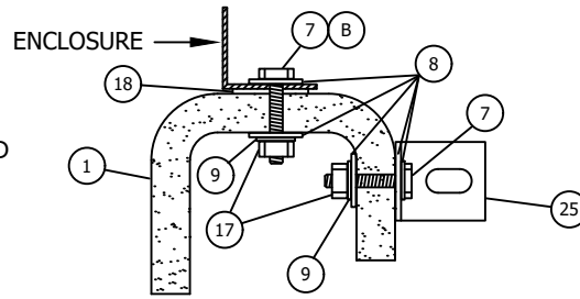
HOLD-DOWN DETAIL AND RING BUSS SUPPORT
