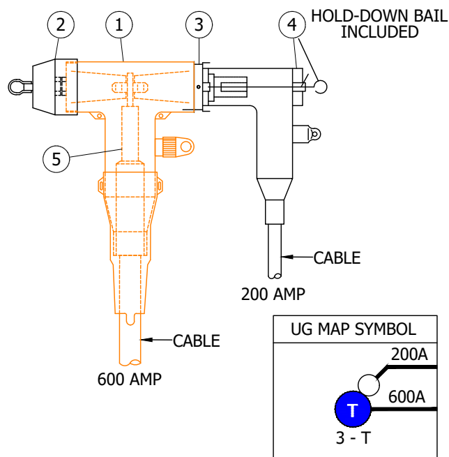
FIGURE 3 MANHOLE INSTALLATION SUBSURFACE CONNECTIONS 200 AND 600 AMP DEADBREAK
