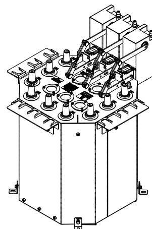
ANGLE VIEW
