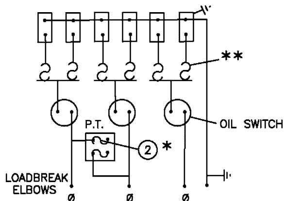
SCHEMATIC DIAGRAM
