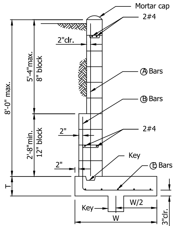
TYPICAL SECTION over 5'-4"
