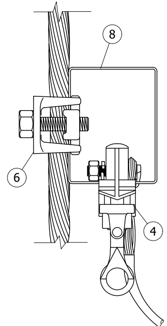
DETAIL 6 OPTION 2
