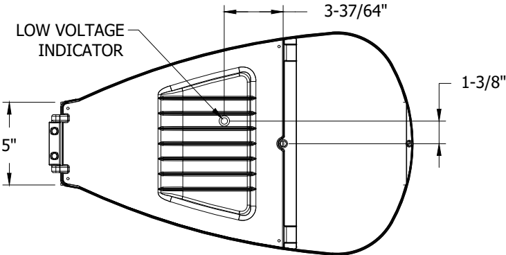
FIGURE 24 BOTTOM VIEW
