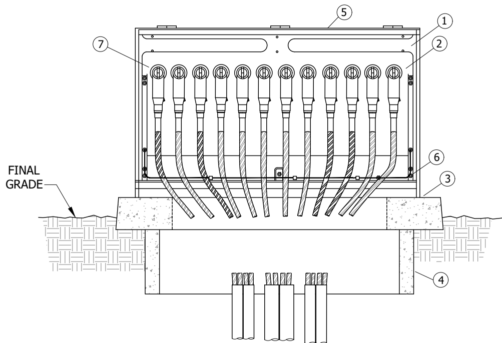
FIGURE 2 200 AMP FRONT VIEW
