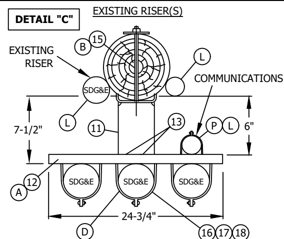
NEW MULTIPLE RISER CONSTRUCTION WITH RISER(S) ON POLE (SEE NOTE (J))
