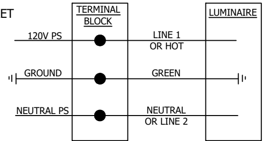
DIAGRAM 1 WIRING SCHEMATIC
