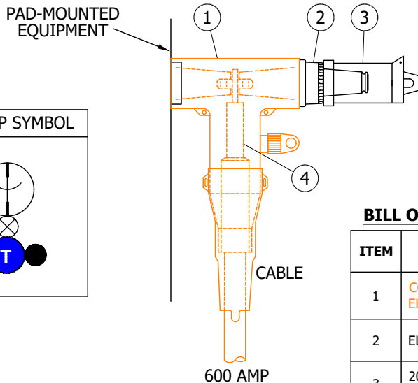
FIGURE 4 PAD-MOUNTED 200/600 AMP EQUIPMENT CONNECTIONS 200 AMP LOADBREAK
