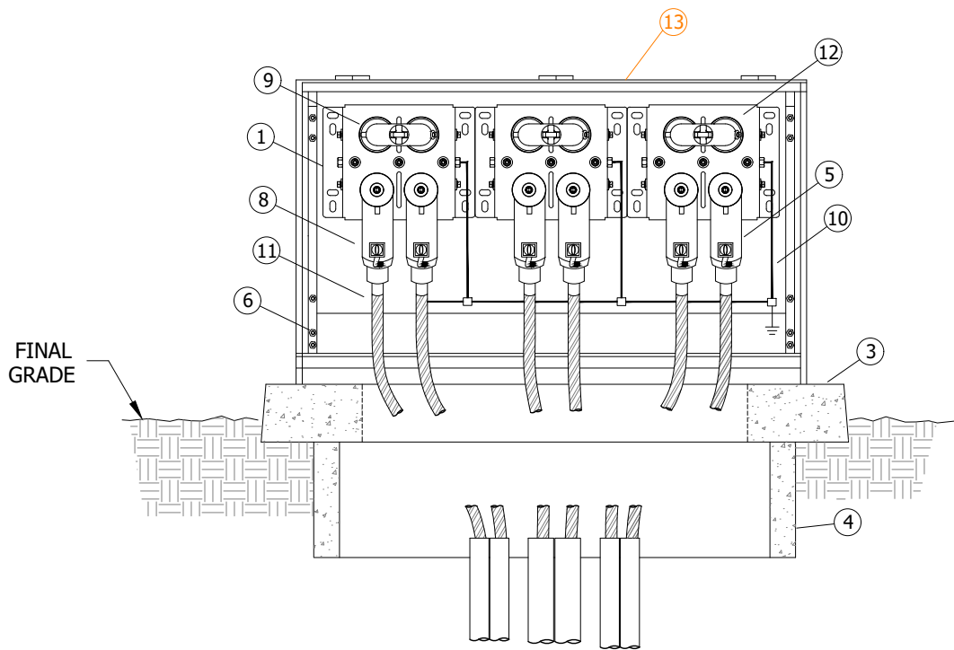
FIGURE 2 600 AMP FRONT VIEW
