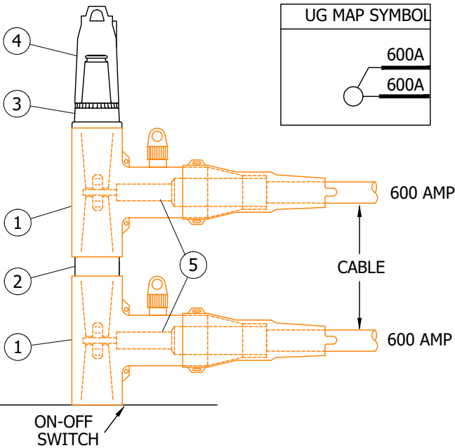
FIGURE 5 SUBSURFACE/SURFACE OPERABLE ON-OFF SWITCH 200 AMP LOADBREAK CONNECTIONS
