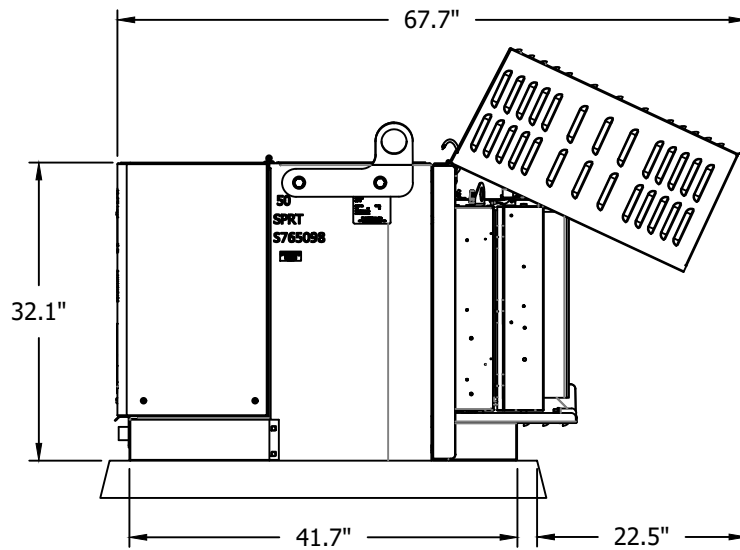
SIDE VIEW FIGURE 2A
