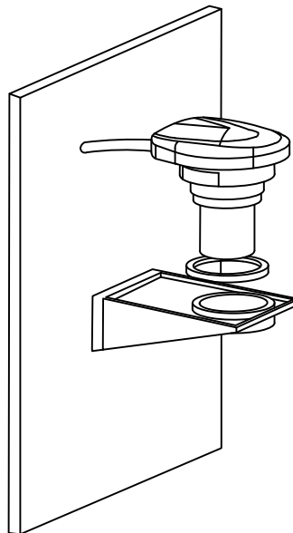
(A) FIGURE 19: INSTALL WDS IN THE MOUNTING BRACKET
