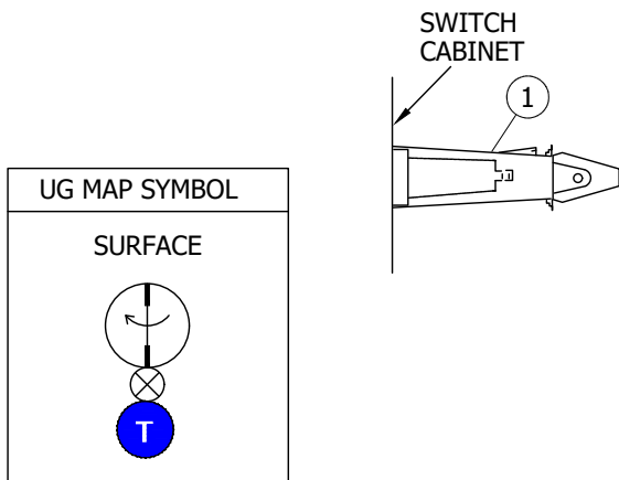
FIGURE 6 SUBSURFACE/SURFACE OPERABLE SWITCH CONNECTIONS 200 AND 600 AMP DEADBREAK
