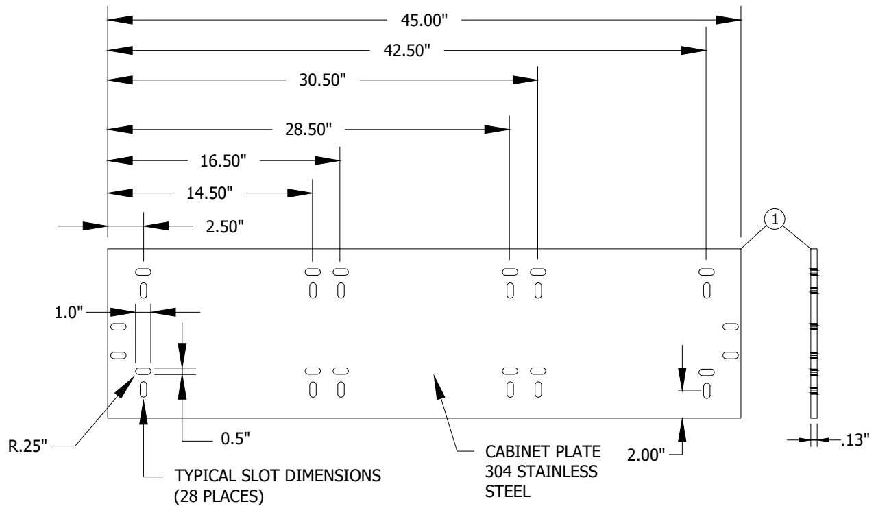
FIGURE 1 600AMP CABINET PLATE ASSEMBLY
