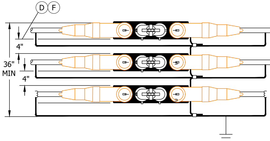
FIGURE 5 IN-LINE BRACKET
