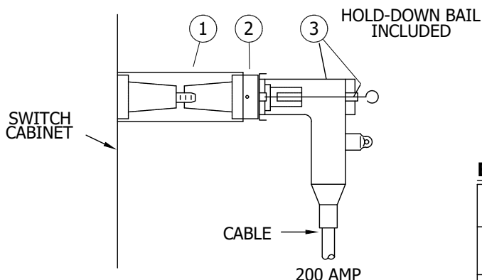
FIGURE 4 SUBSURFACE/SURFACE OPERABLE SWITCH CONNECTIONS 200 AND 600 AMP DEADBREAK
