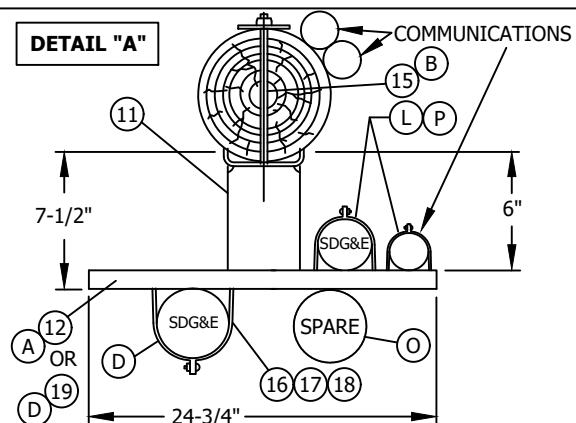
PREFERRED CONSTRUCTION FOR NEW SINGLE RISER WITH AND WITHOUT EXISTING RISER(S) ON POLE (SEE NOTE (G) )
