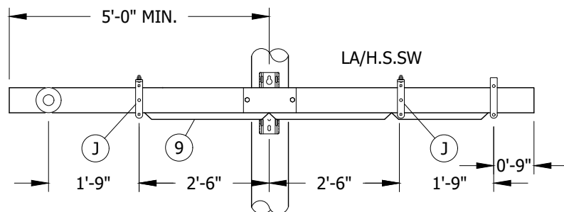
DETAIL 1 FRONT VIEW CONDUIT WITH CABLE SUPPORT BRACKETS
