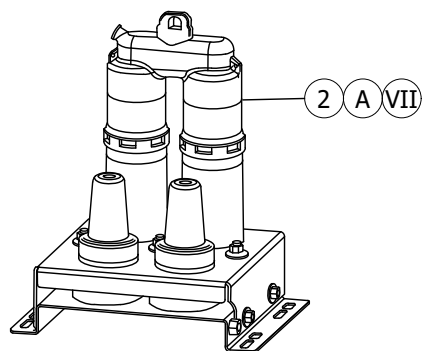
FIGURE 2 SQUARE BRACKET
