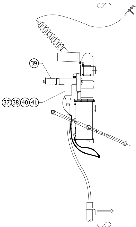
FIGURE 2 600 AMP SIDE VIEW
