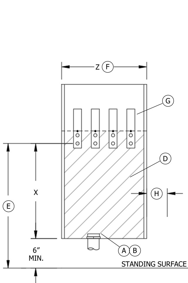
FIGURE 1 FRONT VIEW
