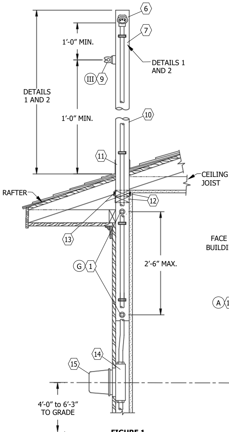
FIGURE 1 SEE TABLE 1
