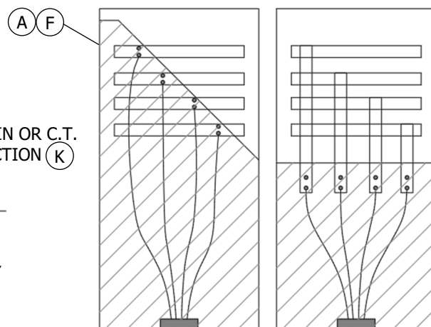
FIGURE 1 PULL SECTION 4,000A MAXIMUM (B) (C) (D) BOTTOM FEED ONLY SEE TABLE 1 FIGURE 2 PULL SECTION 2,000A MAXIMUM (B) (C) (D) BOTTOM FEED ONLY SEE TABLE 1
