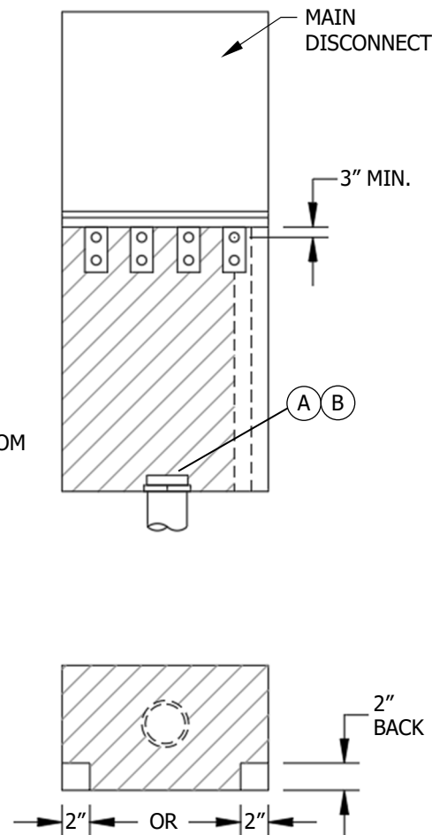
FIGURE 2 COMBINATION UNDERGROUND PULL AND DISCONNECT CAN (C) (L)
