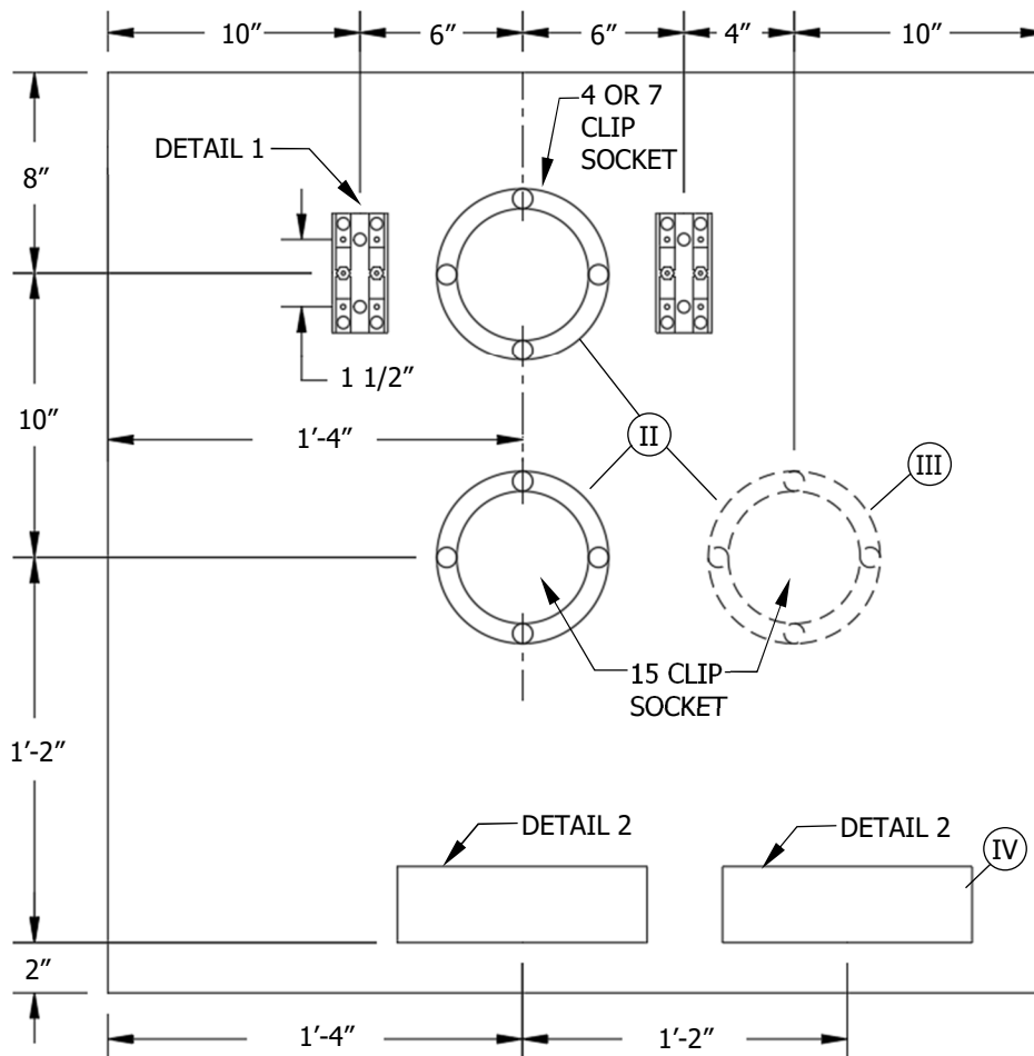
FIGURE 1 METER PANEL LAYOUT
