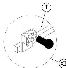
DETAIL 1 NO. 6 - 250 KCMIL GROUND LUG
