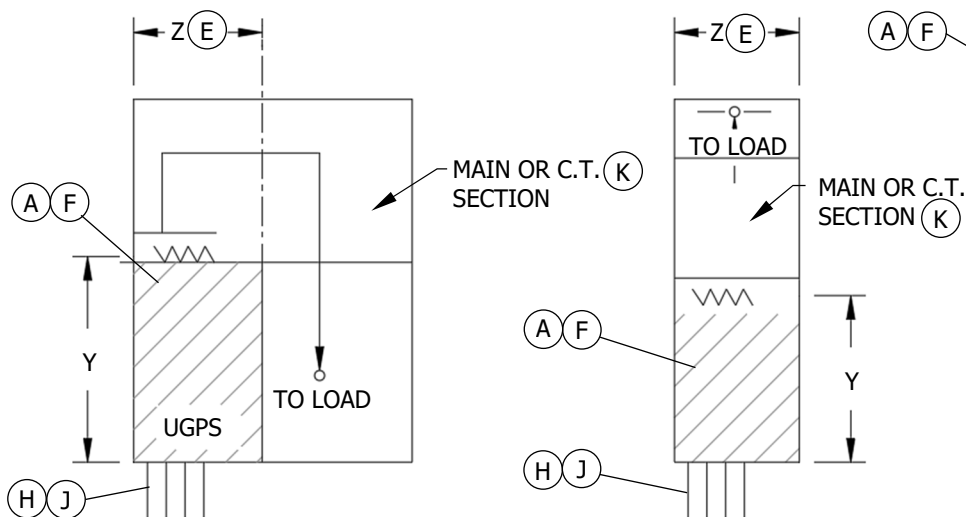
FIGURE 1 PULL SECTION 4,000A MAXIMUM (B) (C) (D) BOTTOM FEED ONLY SEE TABLE 1 FIGURE 2 PULL SECTION 2,000A MAXIMUM (B) (C) (D) BOTTOM FEED ONLY SEE TABLE 1
