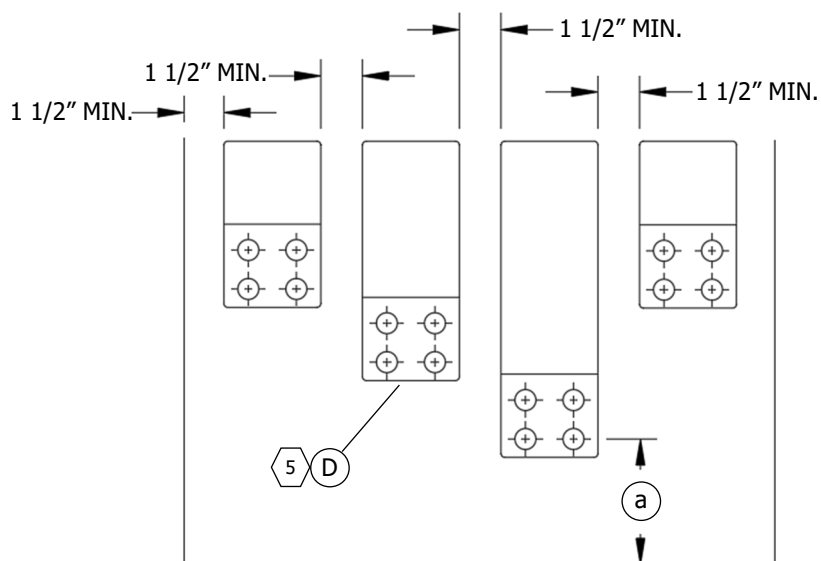
FIGURE 5 SPACING REQUIREMENTS FOR TOP TO BOTTOM STAGGER OF TERMINATING FACILITIES FRONT VIEW
