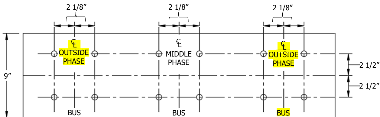
FIGURE 1 CURRENT TRANSFORMER MOUNTING BASE (I)
