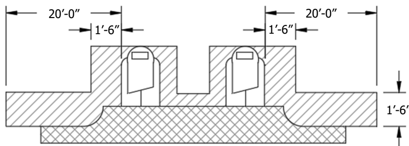
FIGURE 1 FRONT VIEW
