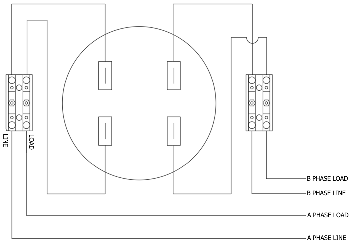
FIGURE 1 CONTROL POWER TRANSFORMER (CPT) METER (I) WIRING DIAGRAM
