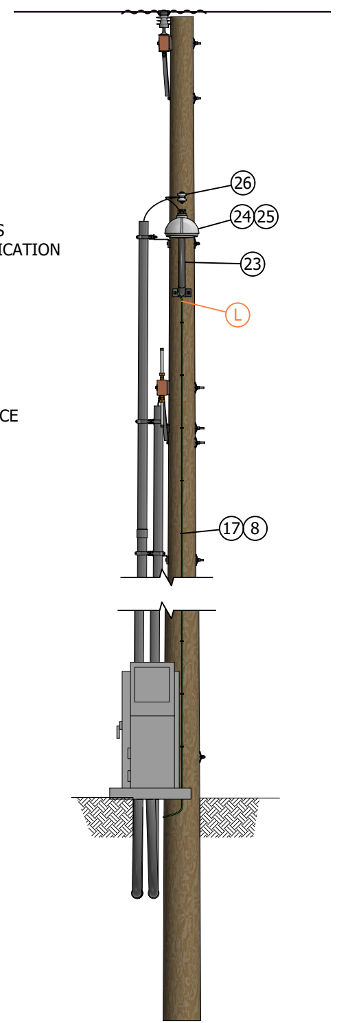
FIGURE 1 SIDE VIEW
