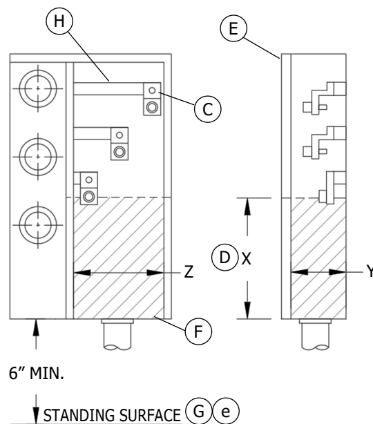
FIGURE 2 (I) FRONT VIEW SEE TABLE 1
