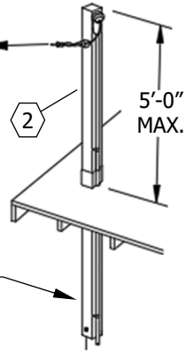
DETAIL 1 SEE TABLE 1
