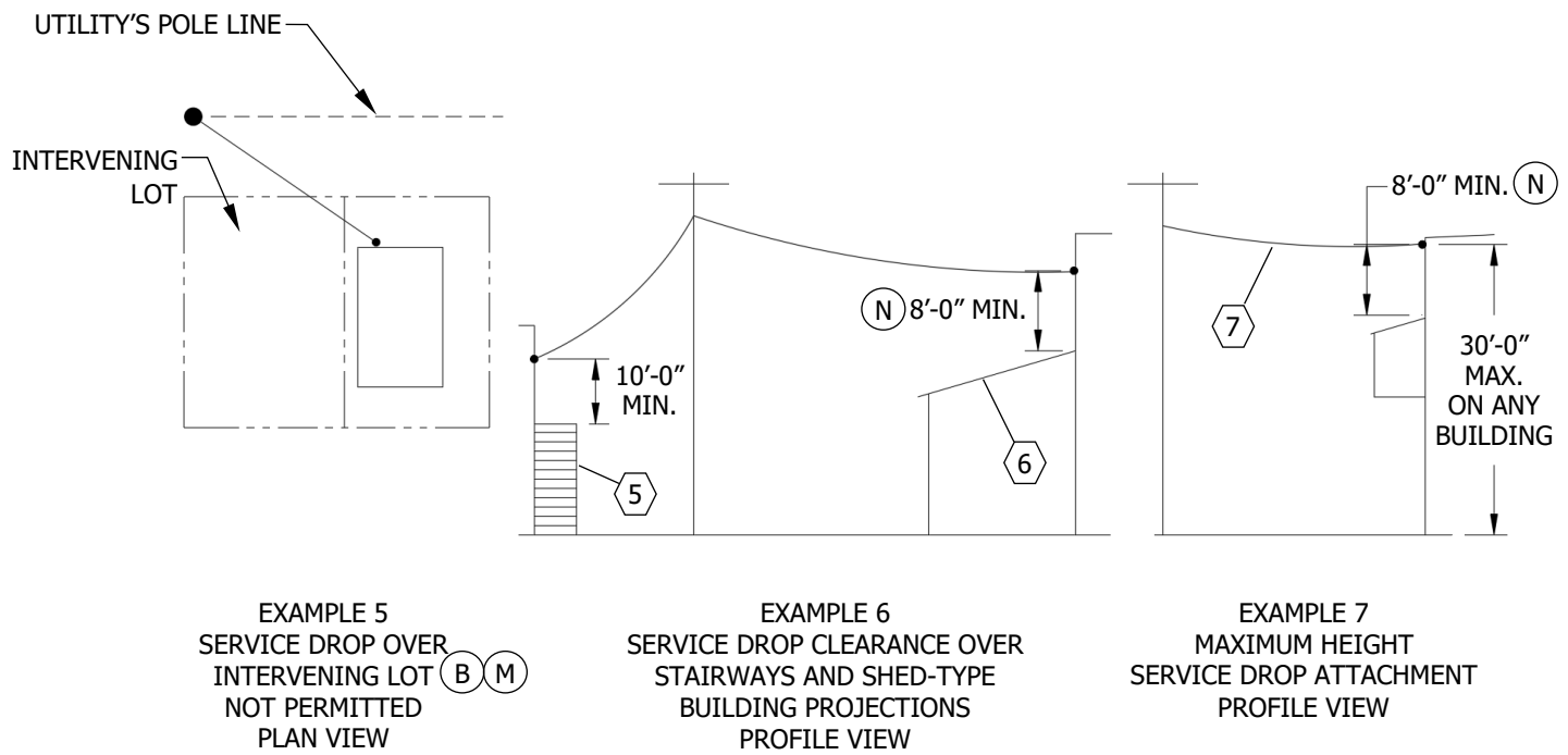
FIGURE 4 (CONT'D) COMMERCIAL AND INDUSTRIAL BUILDINGS OR STRUCTURES SEE TABLE 1
