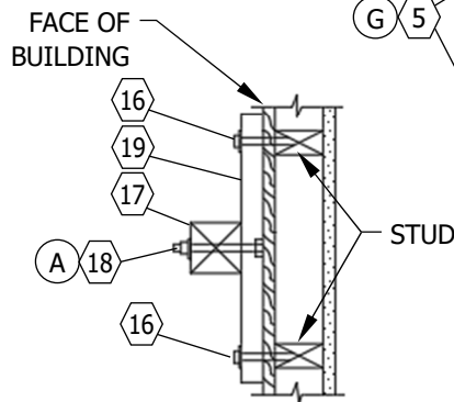
FIGURE 3 ALTERNATE METHOD OF SECURING RISER PLAN VIEW
