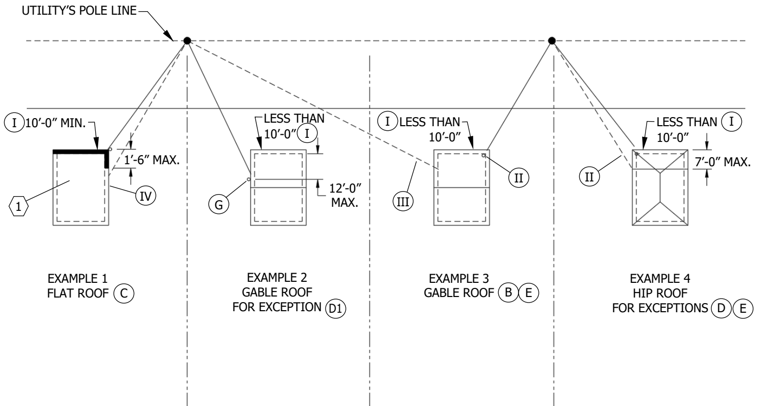
FIGURE 1 RESIDENTIAL BUILDINGS OR STRUCTURES PLAN VIEW SEE TABLE 1
