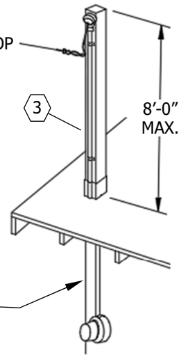
DETAIL 2 SEE TABLE 1 (F)
