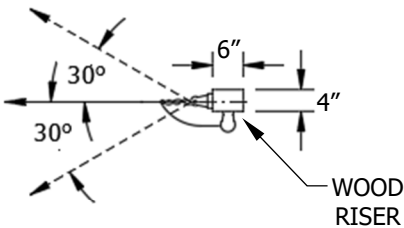
DETAIL 1 PLAN VIEW SEE TABLE 1 (B)
