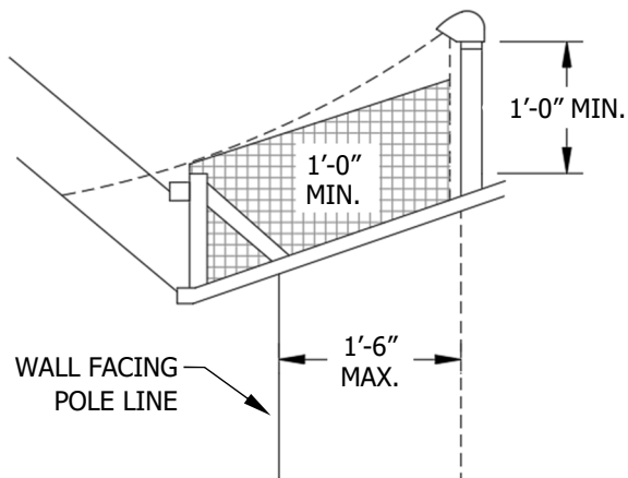
EXAMPLE 5 FLAT OR SLOPING EAVE OR ROOF
