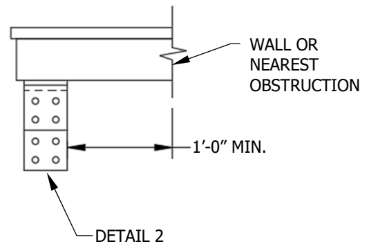
CONFIGURATION 2 STUBS STAGGERED VERTICALLY SIDE VIEW
