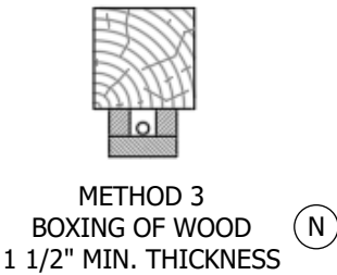
FIGURE 2 ALTERNATE METHODS OF COVERING SERVICE ENTRANCE CONDUITS (M)
