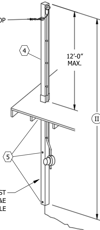
DETAIL 3 SEE TABLE 1
