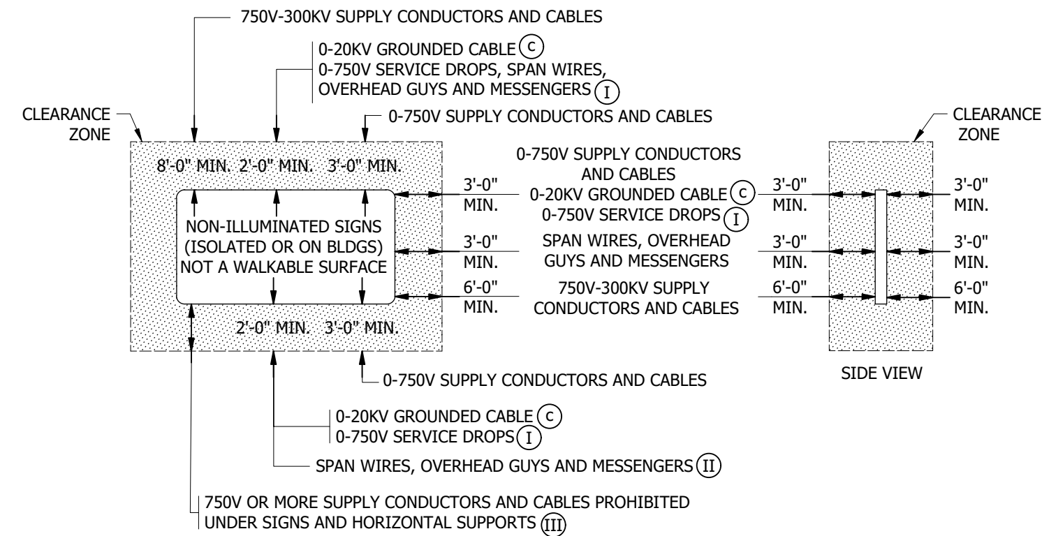
FIGURE 4 CLEARANCES FROM NON-WALKABLE NON-ILLUMINATED SIGNS
