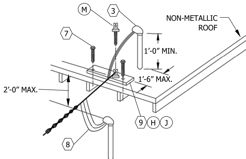
EXAMPLE 6 WOOD REINFORCING BLOCK
