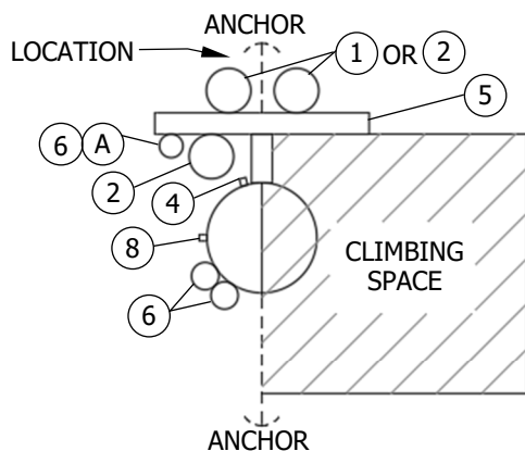
CONFIGURATION 1 DEADEND MULTIPLE POWER RISER
