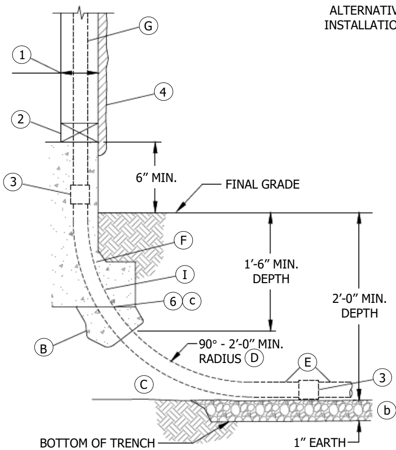
FIGURE 1 TYPICAL ELEVATION
