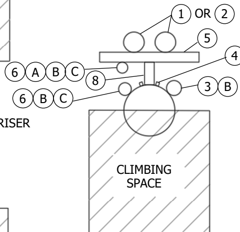
FIGURE 3 NEW CONSTRUCTION WITH EXISTING SDG&E RISER DEADEND OR THROUGH CONSTRUCTION MULTIPLE RISER
