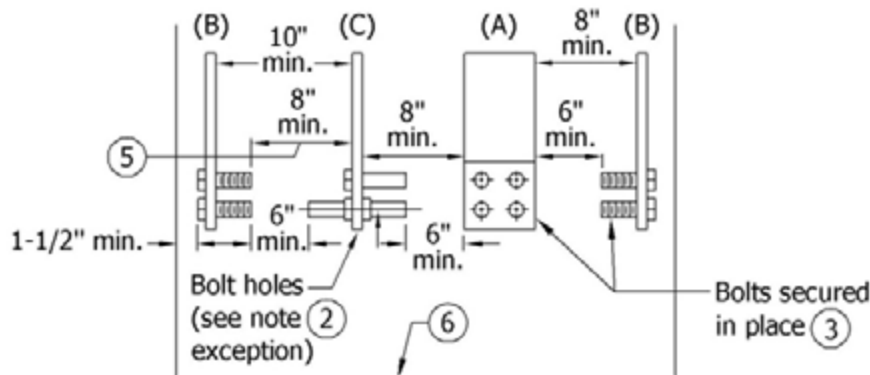
FIGURE 3 Spacing requirements for terminating facilities accessible from (A) front only, (B) one side only, or (C) from either side. ③ ④
