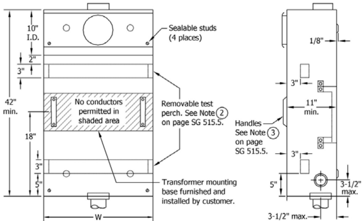
Minimum Box Dimensions
