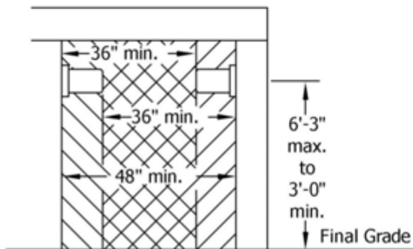
FIGURE 3 - Side View
