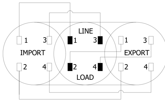
METERING ADAPTER (TYPICAL)
