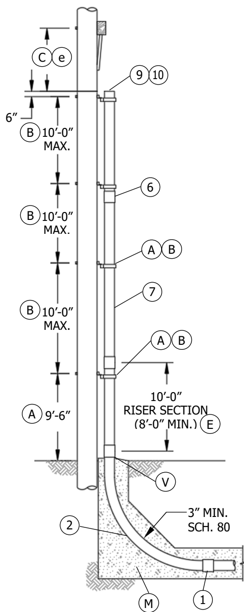
FIGURE 1 (N) SIDE VIEW
