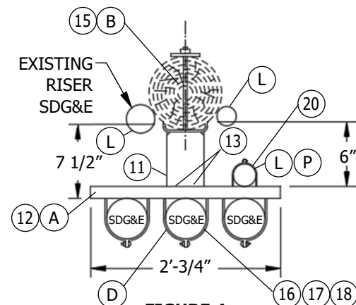
FIGURE 4 EXISTING RISER(S) NEW MULTIPLE RISER CONSTRUCTION WITH RISER(S) ON POLE (J)
