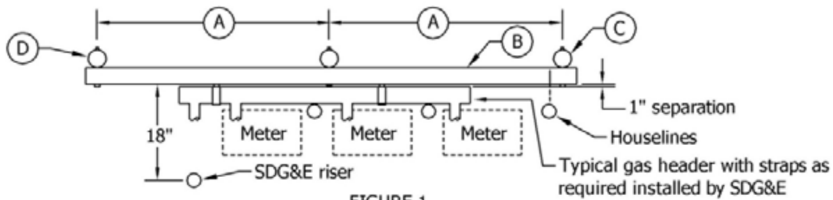
FIGURE 1 Top View
