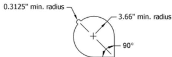
FIGURE 3 Meter Panel Cover Cutout Detail
