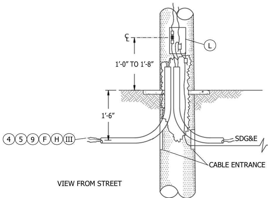
EXAMPLE 1 DIRECT BURIED POLE
