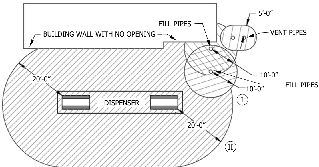
FIGURE 1 PLAN VIEW
