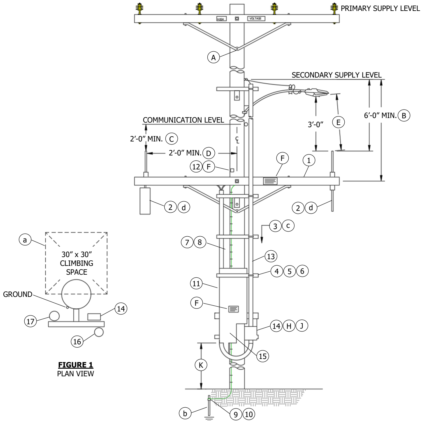
FIGURE 1 UNMETERED (UM) ELECTRIC SERVICE FROM AN OVERHEAD SOURCE
