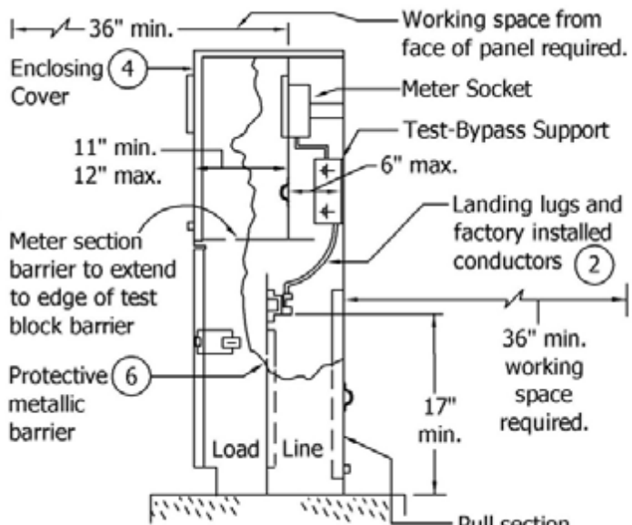
FIGURE 2 Side View (Typical) See (1) & (2)
