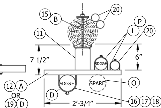
FIGURE 2 PREFERRED CONSTRUCTION FOR NEW SINGLE RISER WITH OR WITHOUT EXISTING RISER(S) ON POLE (G)
