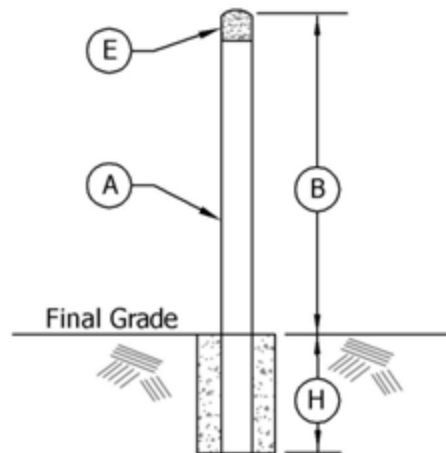
Heavy Duty and Light Duty Barricade Posts Concrete Footing
