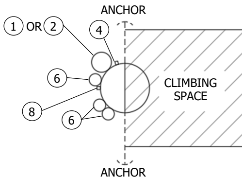
CONFIGURATION 1 DEADEND SINGLE POWER RISER
