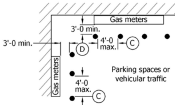
Barricades for New Gas Meter Installations Commercial or Multi-Family (More Than 2 Units)
