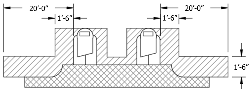
FIGURE 1 FRONT VIEW
