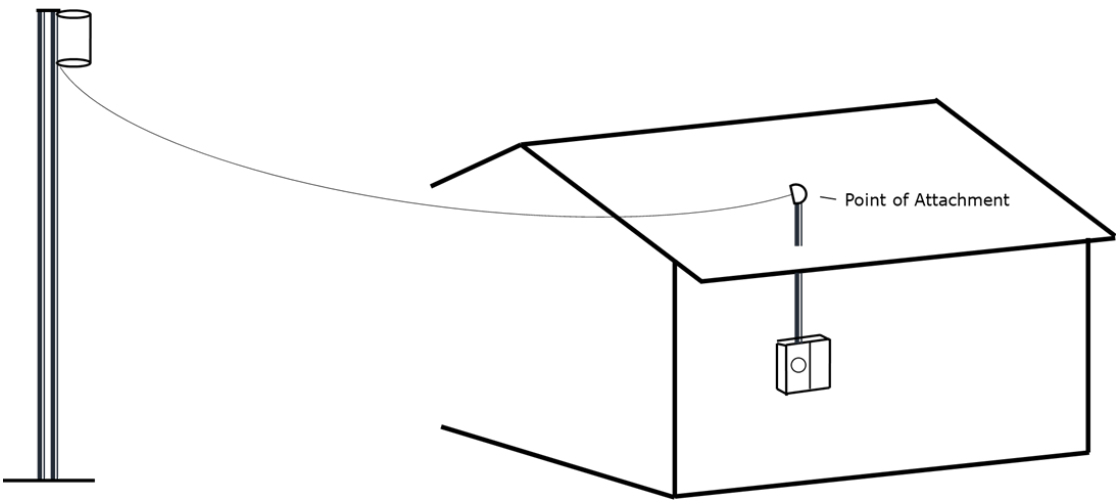
FIGURE 2: Direct Feed into Service Panel or with use of a Meter Adaptor
